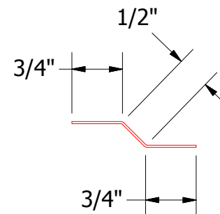
DSA975/DWA975 - Joggle Cleat
