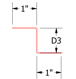
Support Z DWA681: D3=1" DSA681: D3=1 5/8"
