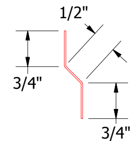
DWA975/DSA975 - Joggle Cleat
