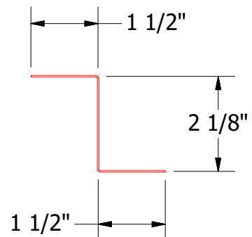
FLA914-Z Closure
