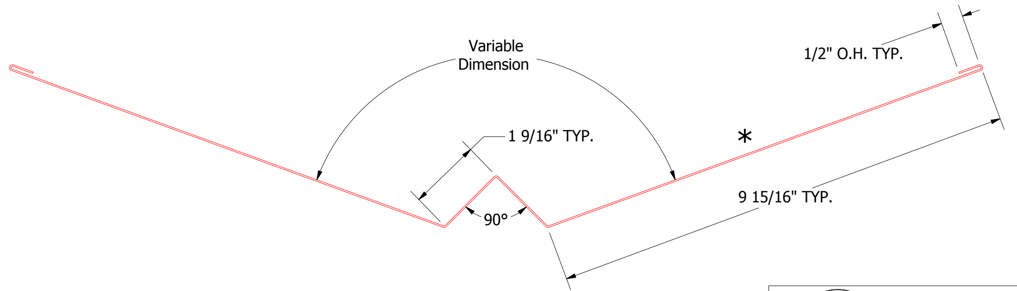
Universal Valley Trim
