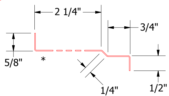
BGA912-Vented Closure Angle
